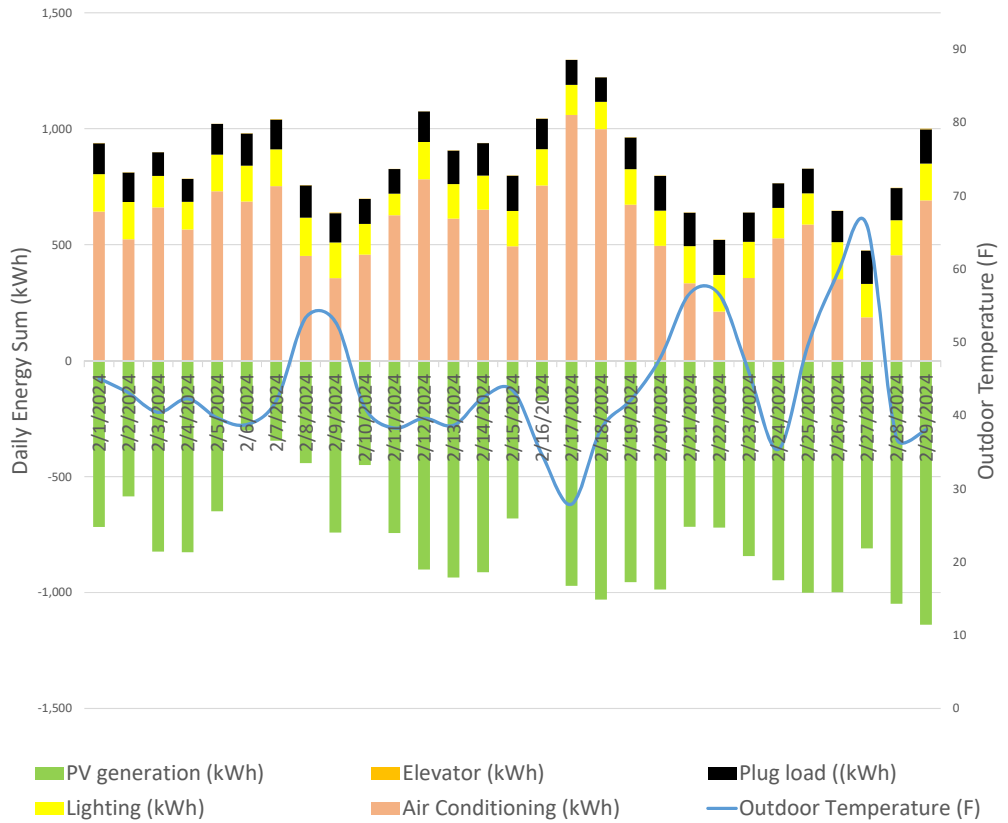
February Daily Energy Results
