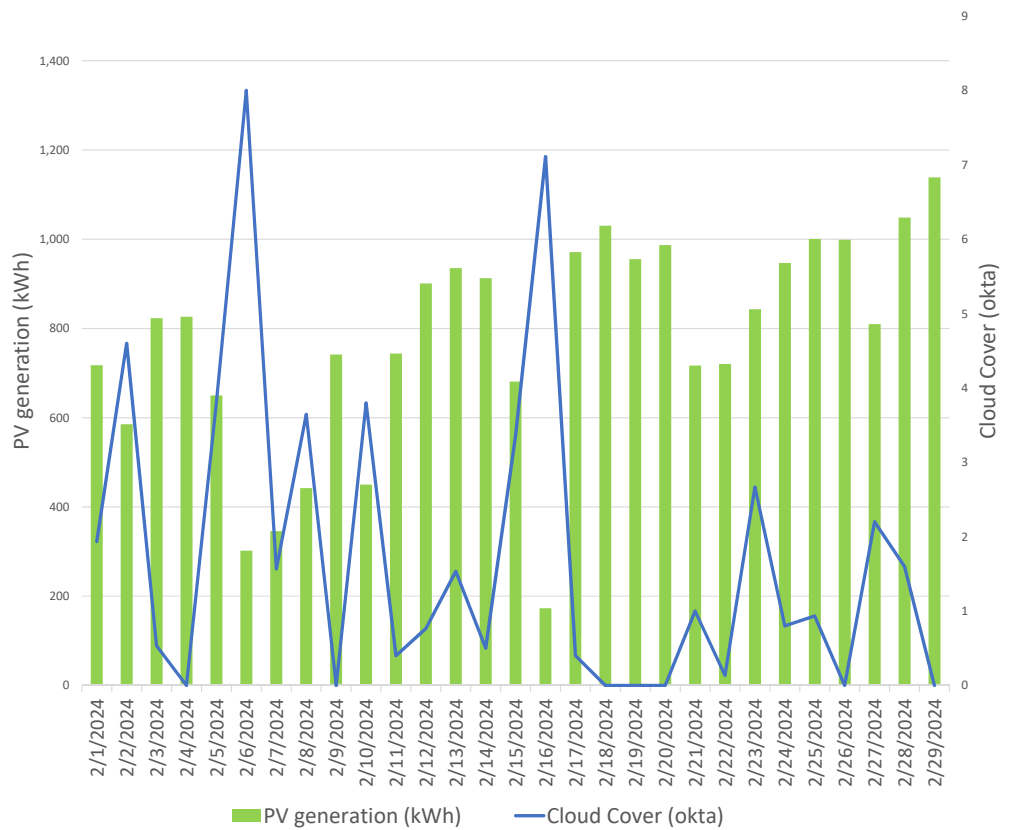
February PV Daily
