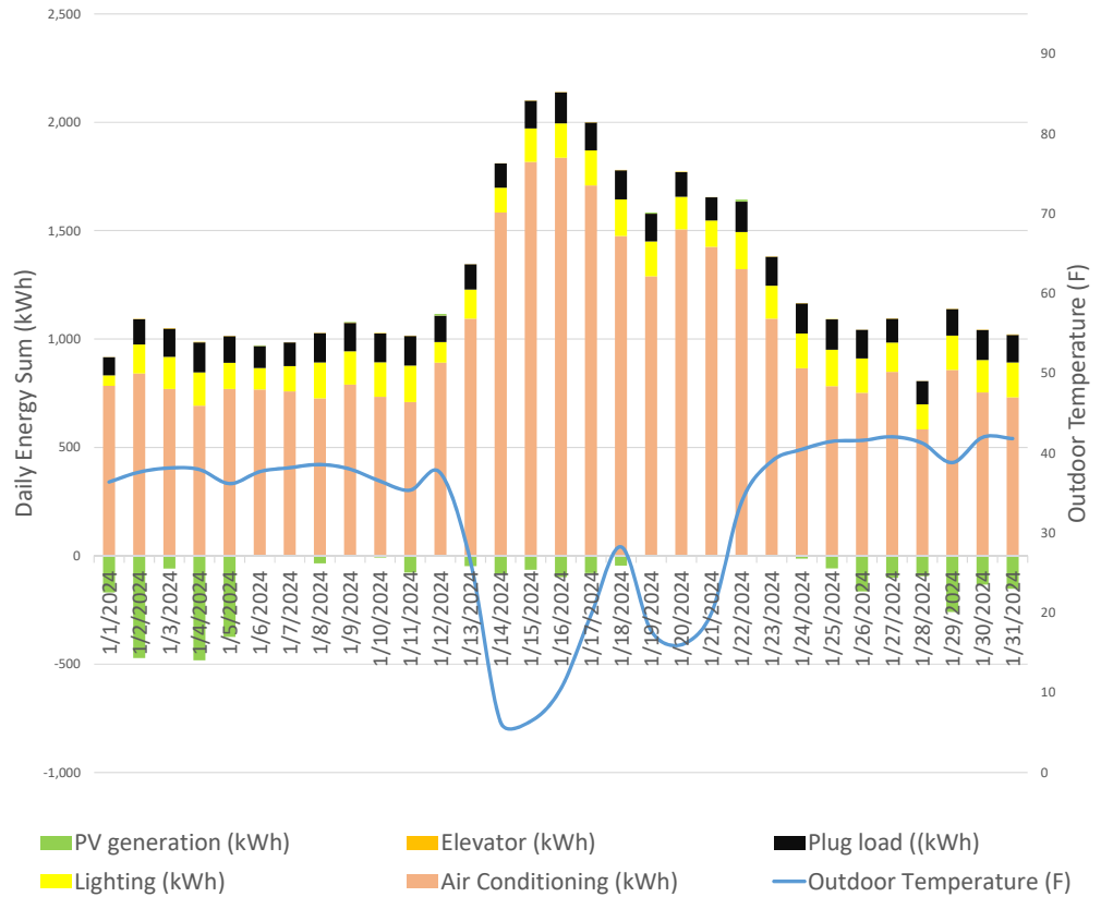
January Daily Energy Results
