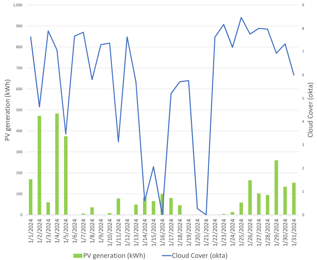
January PV Daily
