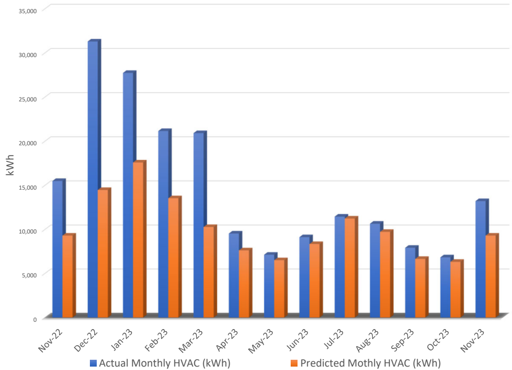
Monthly HVAC (kWh)
