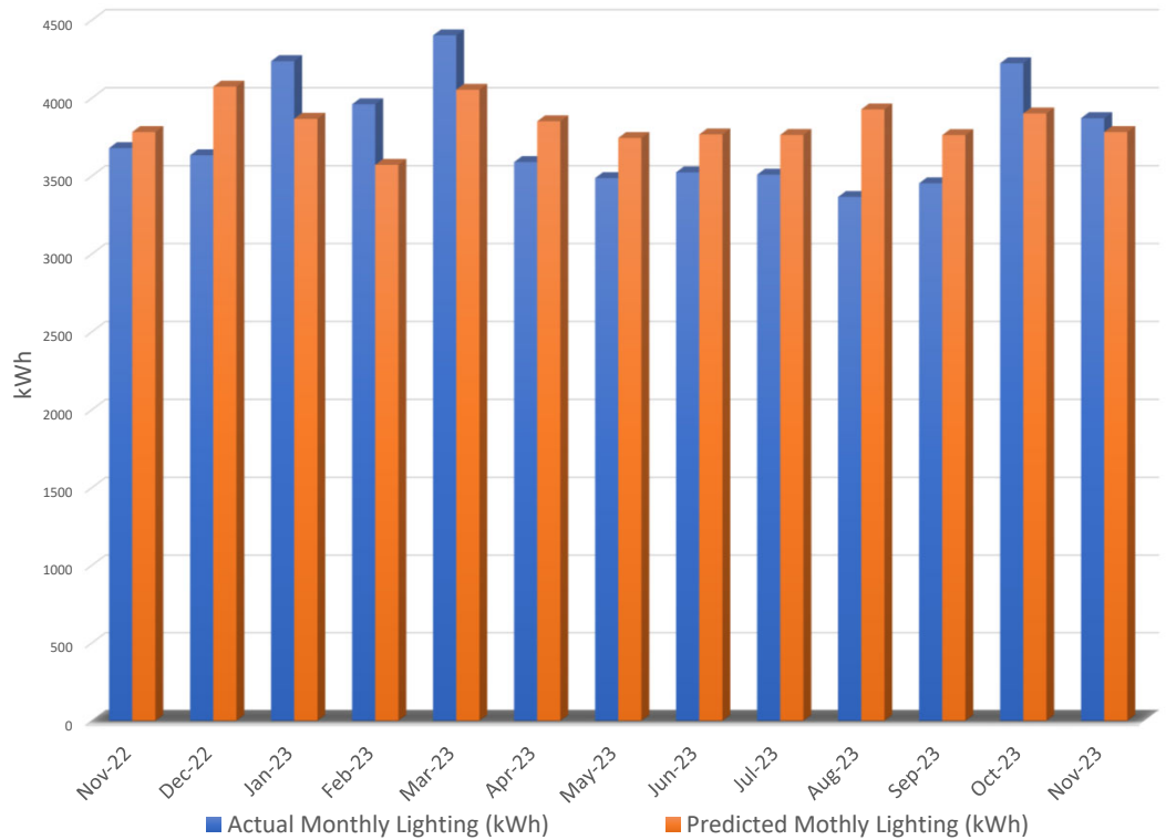
Monthly Lighting (kWh)
