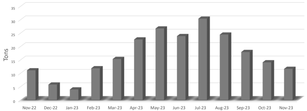
Monthly Equivalent Avoided CO2 Emissions (Tons)
