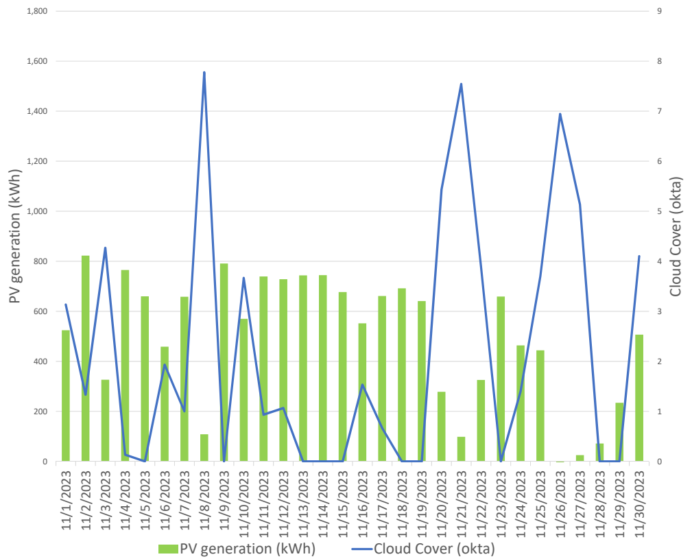
November PV Daily
