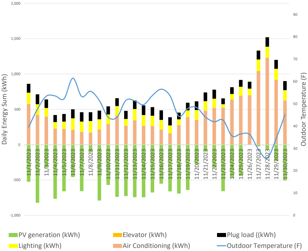
November Daily Energy Results
