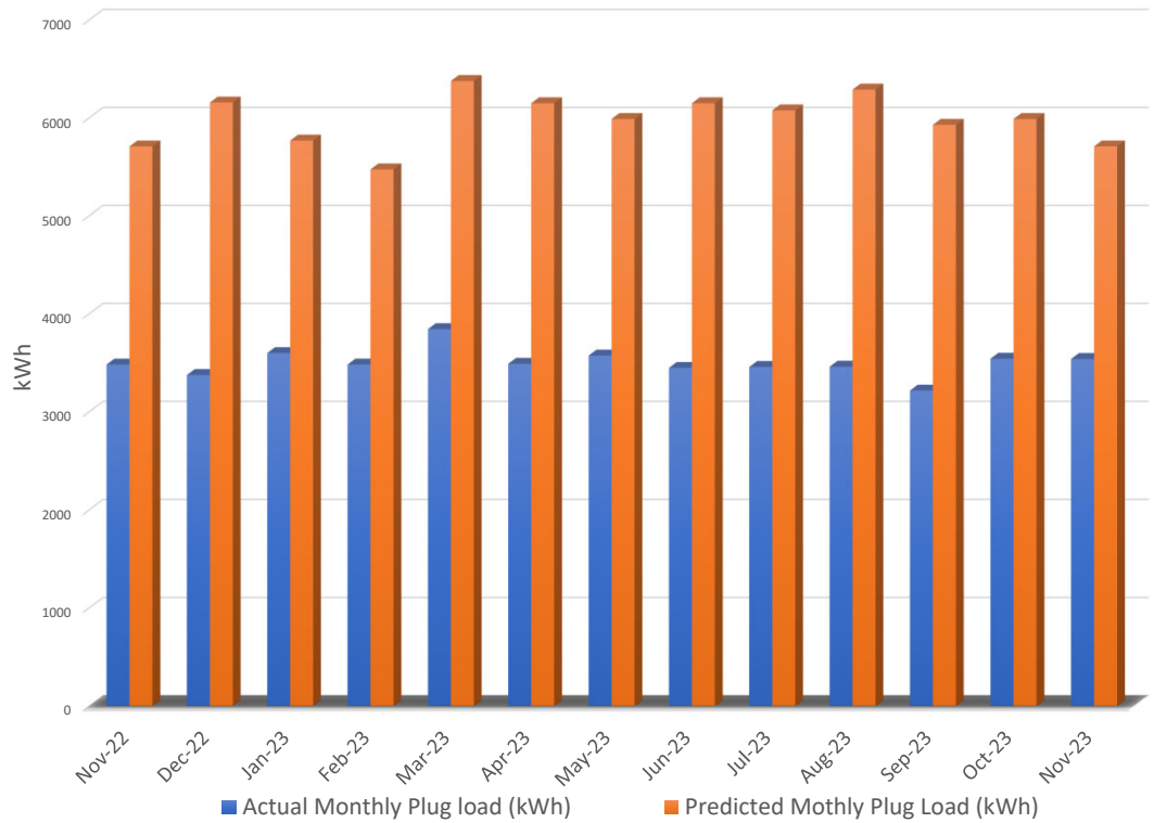
Monthly Plug Load Consumption (kWh)
