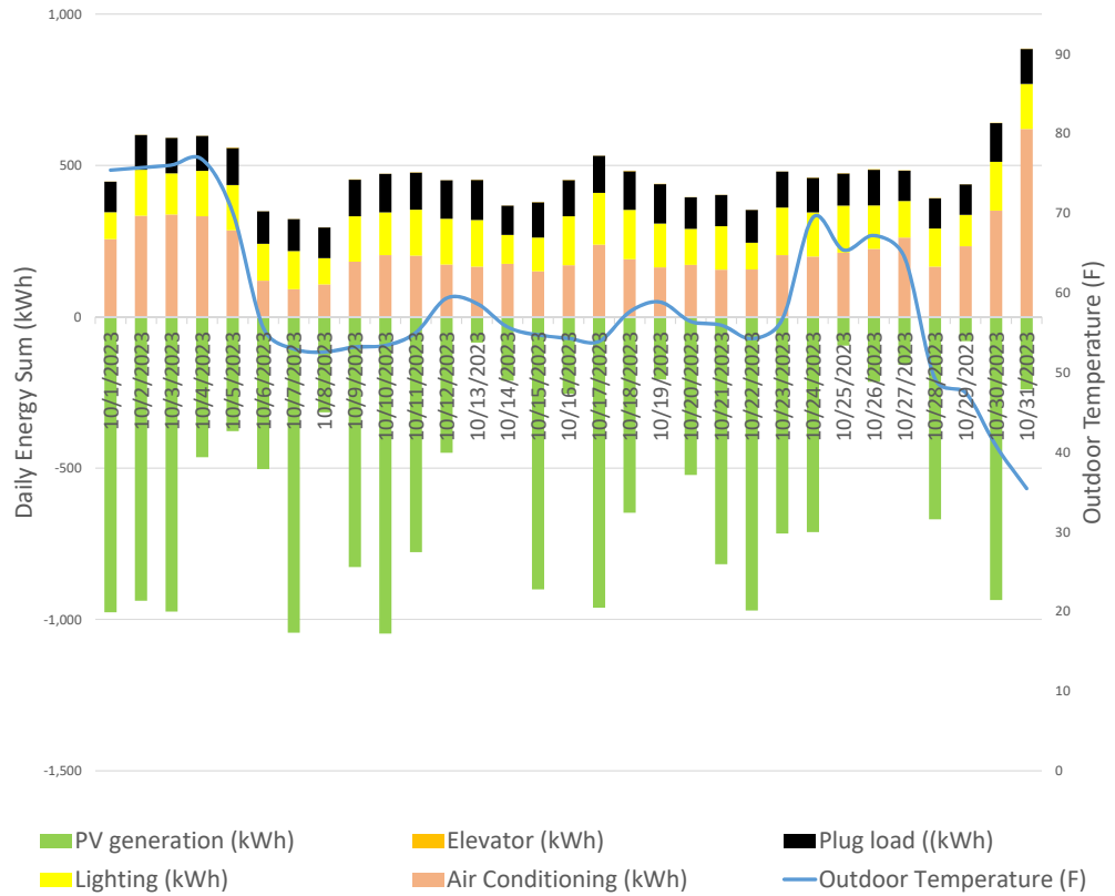
October Daily Energy Results
