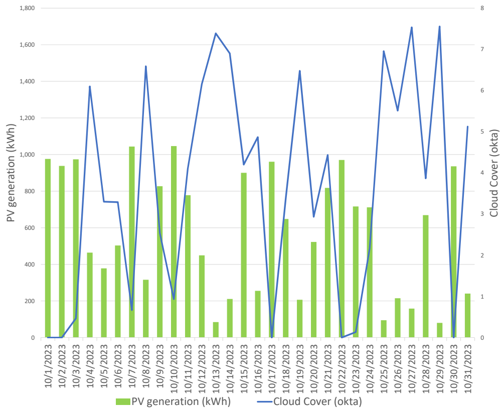
October PV Daily
