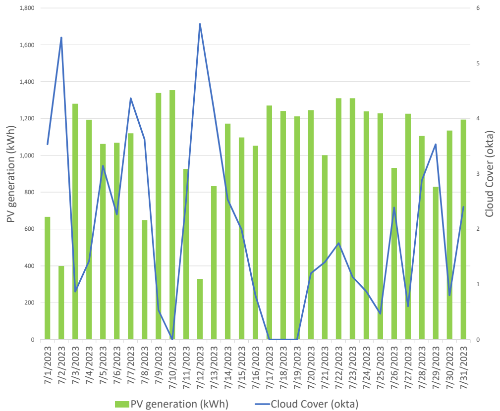
July PV Daily
