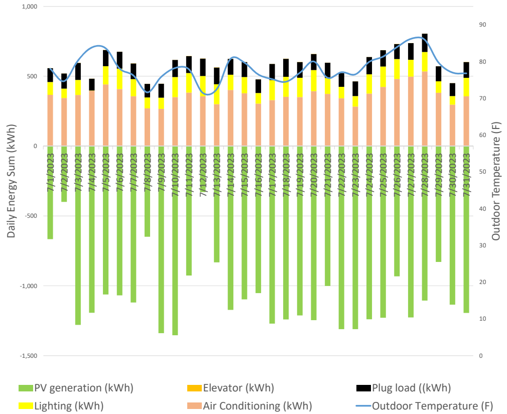
July Daily Energy Results
