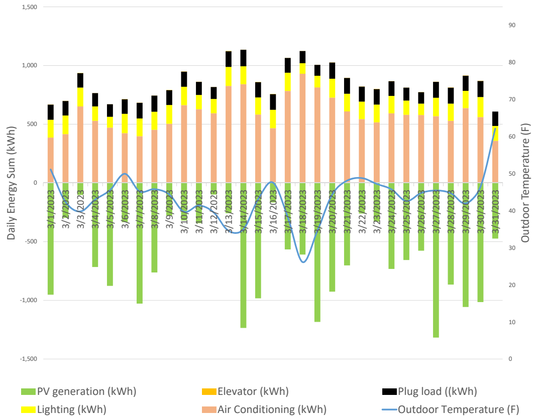
March Daily Energy Results
