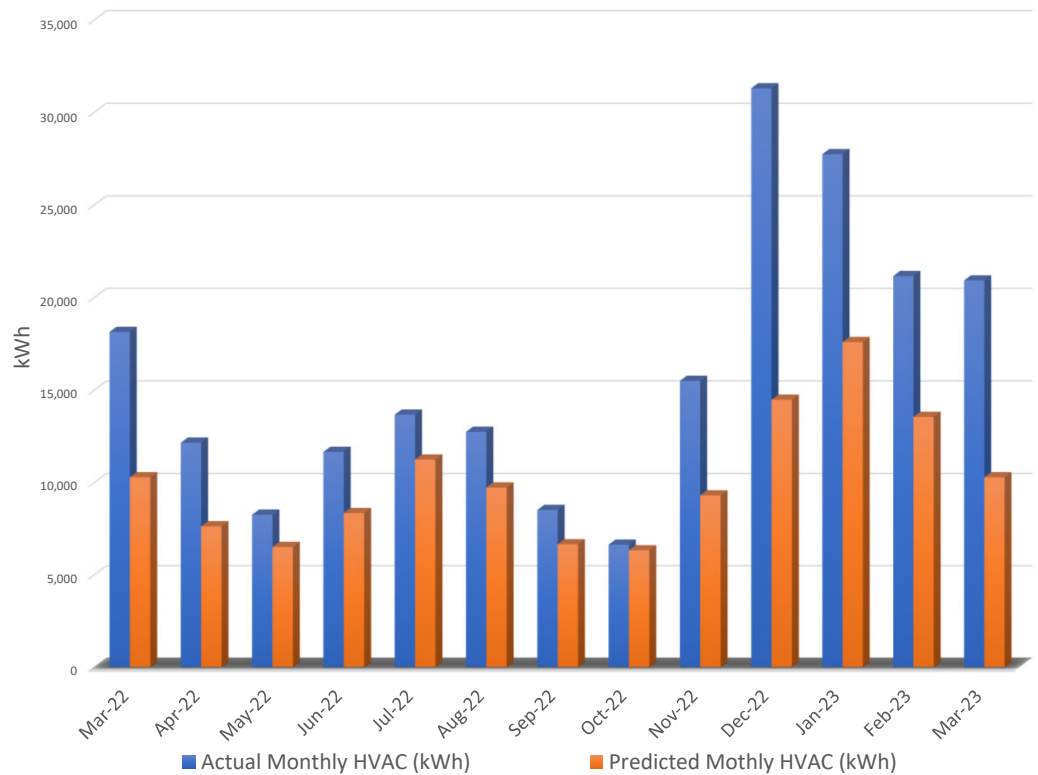
Monthly HVAC (kWh)
