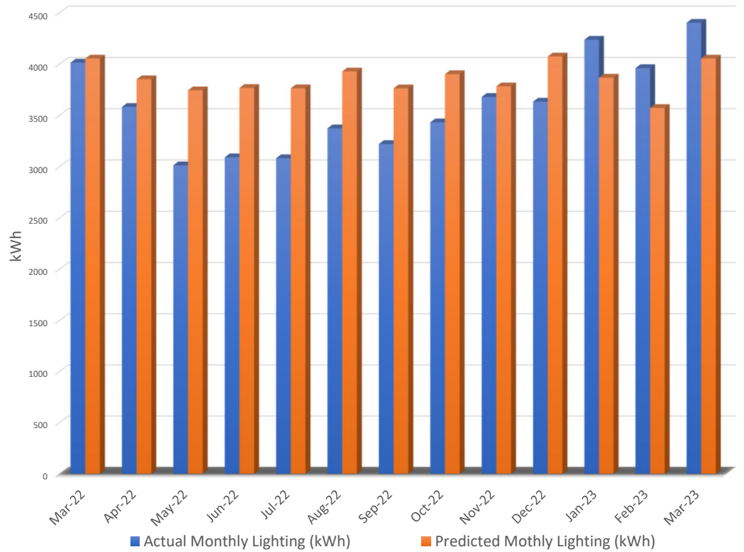
Monthly Lighting (kWh)
