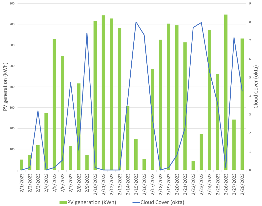
February PV Daily
