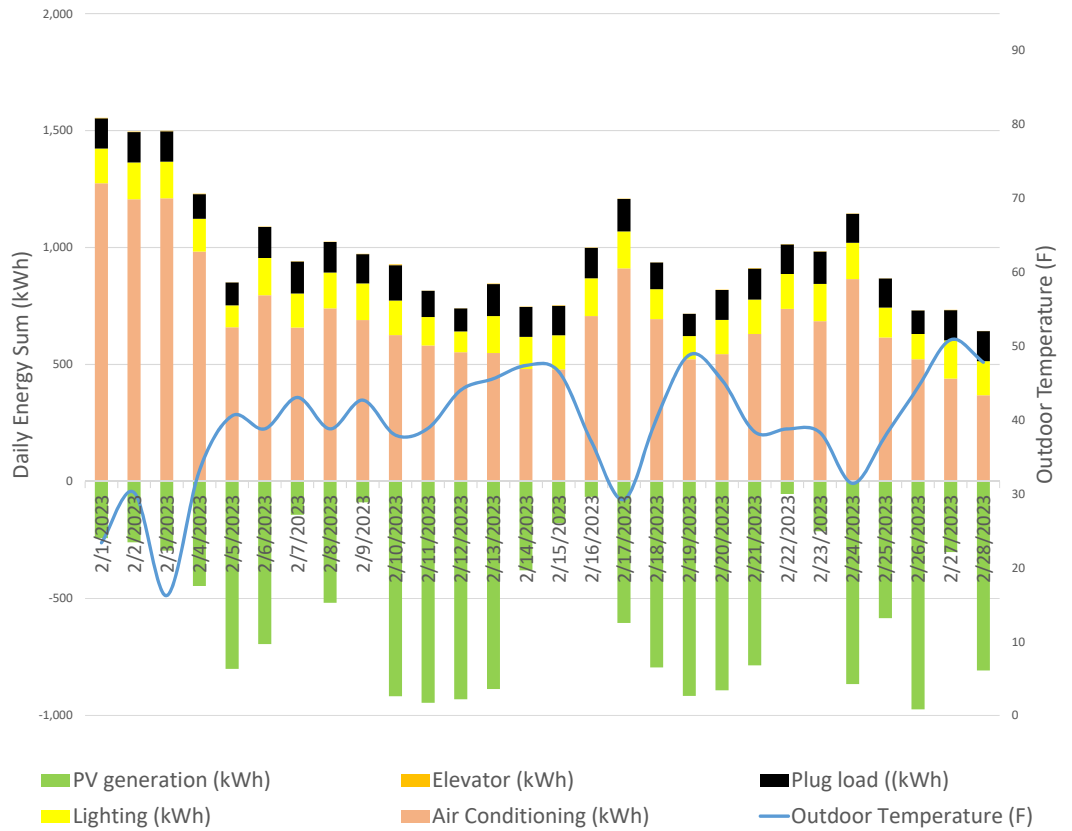
February Daily Energy Results
